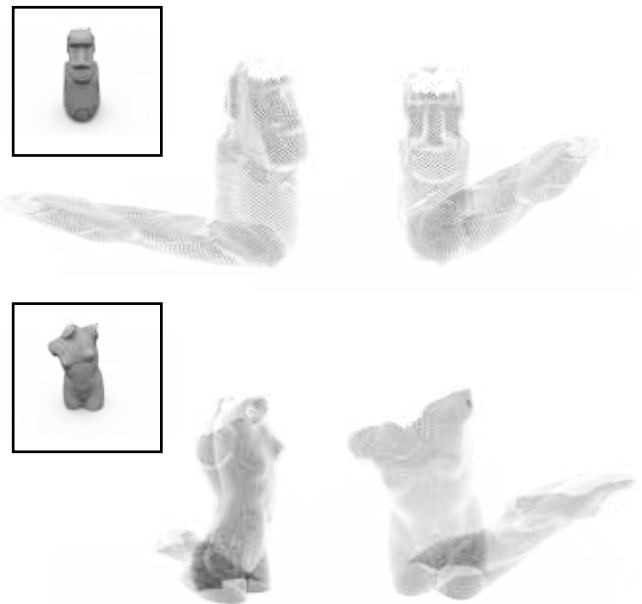
Figure 13: Wire meshes of a Moai statue (top) and a female torso sculpture (bottom), designed using zig-zag initial conditions to account for their cylindrical topologies.
